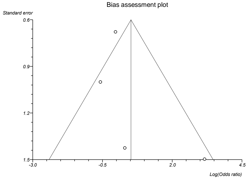
Supplementary Figure 8. L'Abbe, odds ratio, and Bias assessment plots for HTN among CAP patients.
