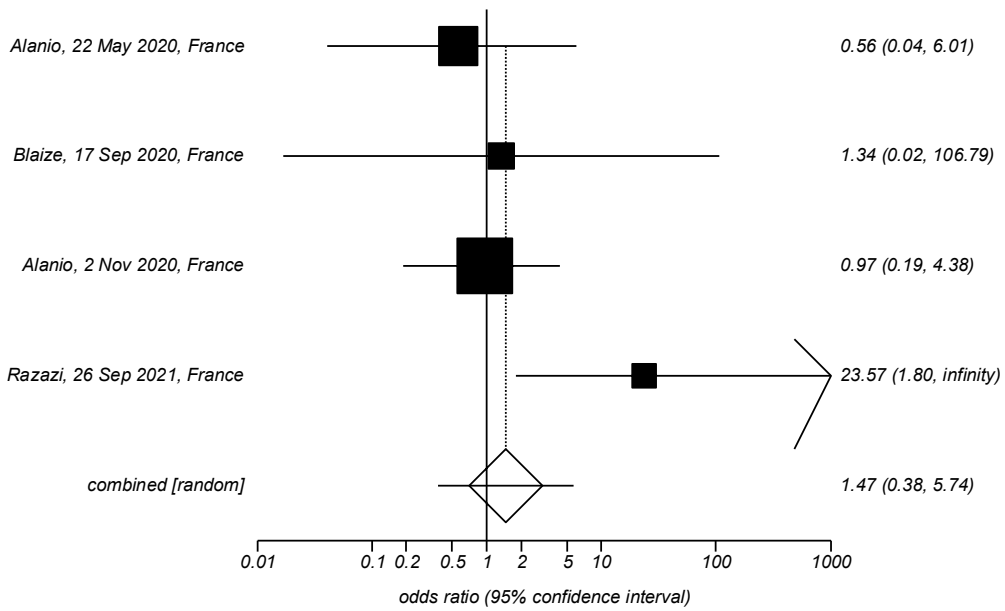
Odds ratio meta-analysis plot [random effects]
