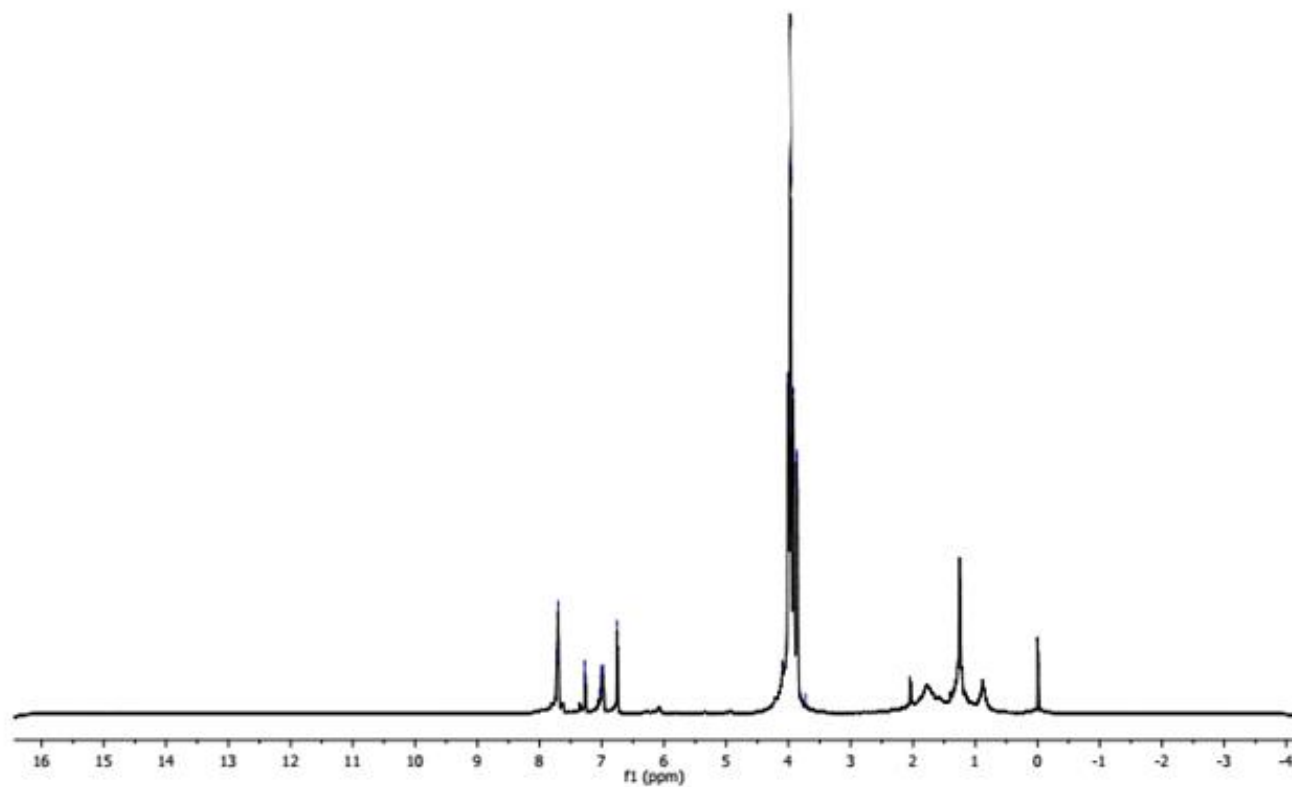
Supplementary Figure 3. ^1\text{H-NMR} spectrum of isolated compound of acetone extract.
